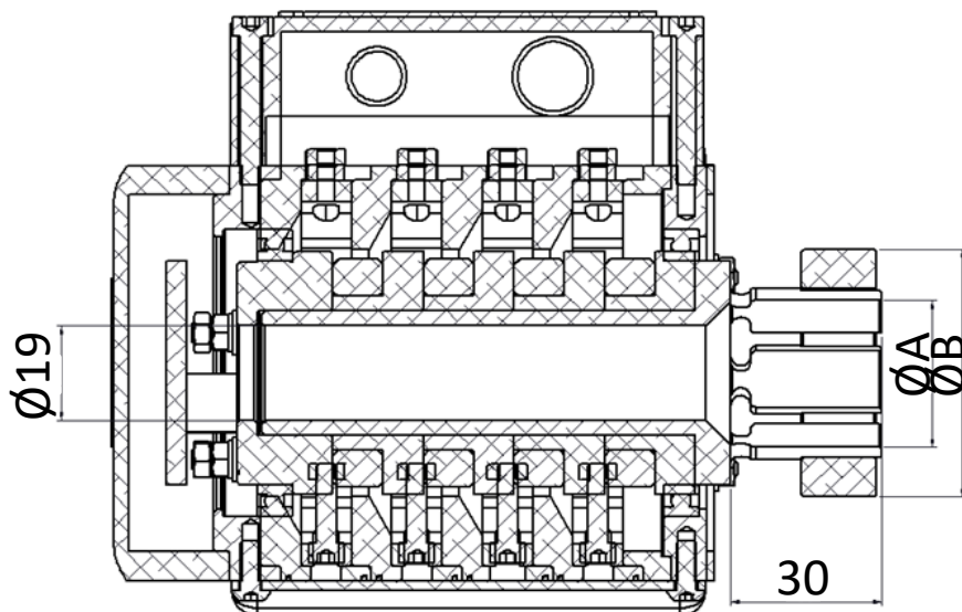
AISI 304 STAINLESS STEEL AXIS
