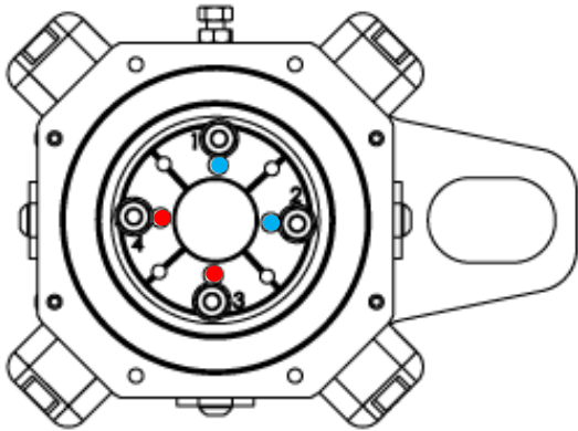
OUTPUT CHANNELS (ROTOR)
